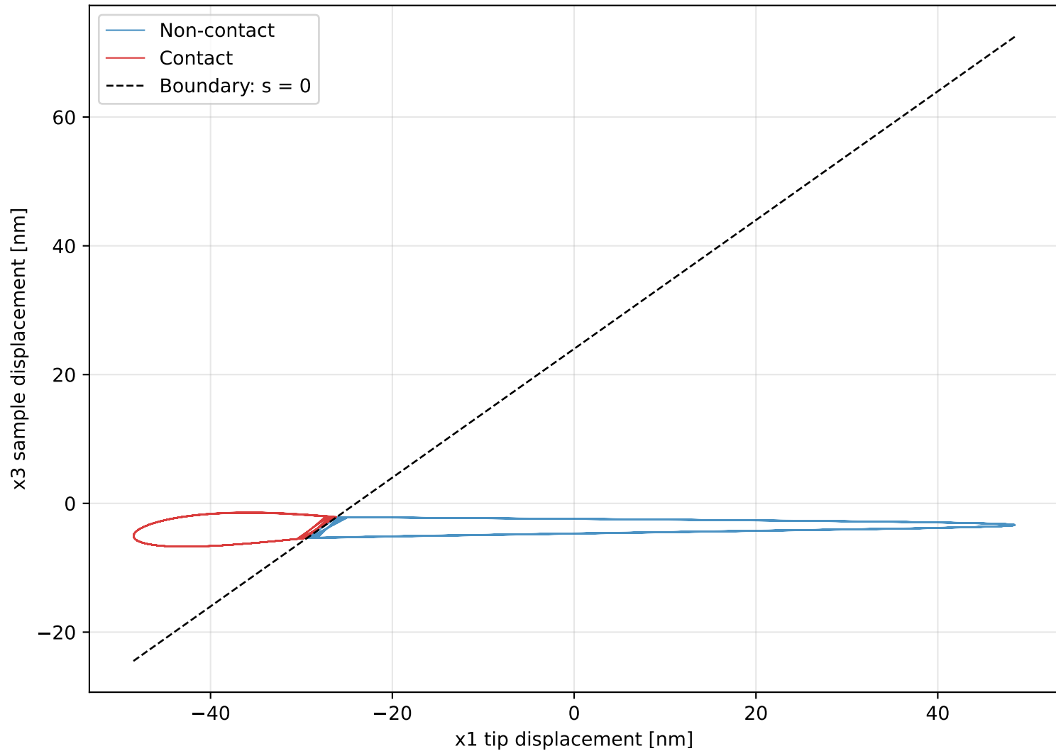
AFM DMT-KV Phase Space: x1 vs x3 (1600-1650 \mu s)
